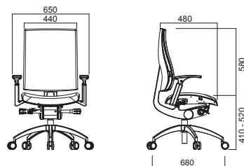
SKILL WITH MESH BACKREST AND SYNCHRON MECHANISM
